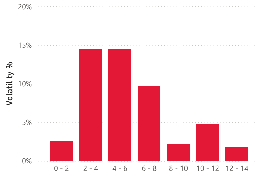
Volatility Distribution
