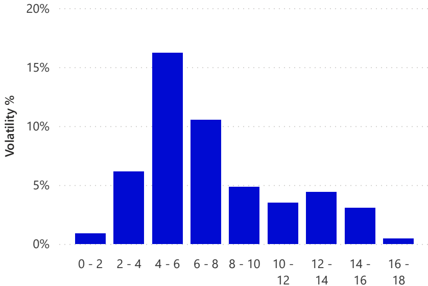
Volatility Distribution
